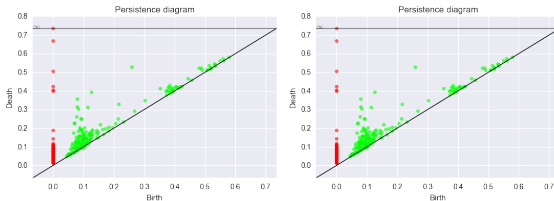
Figure 16: Persistence diagrams for two configurations of MBP.
