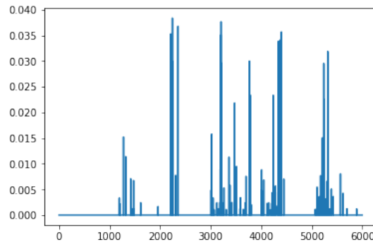
Figure 20: Variable importances of the landscapes coefficients for the classification of Walkers. The 3 000 first coefficients correspond to the three landscapes of dimension 0 and the 3 000 last coefficients to the three landscapes of dimension 1. There are 1000 coefficients per landscape. Note that the first landscape of dimension 0 is always the same using the Rips complex (a trivial landscape) and consequently the corresponding coefficients have a zero importance value.
